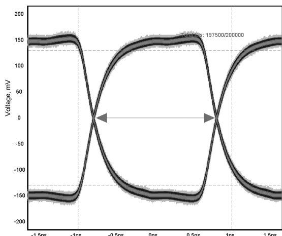
Figure 17. LVDS RxCLKOUT Output (3.125 Gbps, 20m CAT-6 SFTP, 0x001 DS32ELX0124 EQ setting, 0x10 DS32EL0421 De-Emphasis setting)
