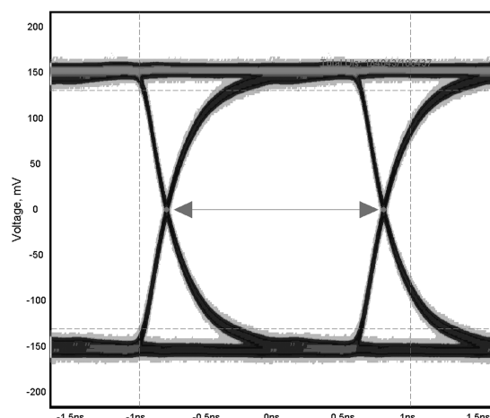
Figure 18. LVDS RxOUT0 Output (3.125 Gbps, 20m CAT-6 SFTP, 0x001 DS32ELX0124 EQ setting, 0x10 DS32EL0421 De-Emphasis setting)
