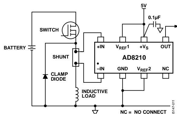
Figure 34. High-Side Switch
