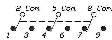
CIRCUIT: 3PDT
