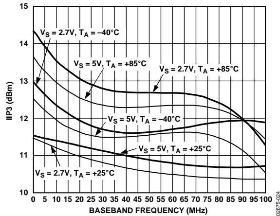
Figure 15. IIP3 vs. F_{BB} , V_{GIN} = 1.2\text{ V} , F_{LO} = 1900\text{ MHz}
