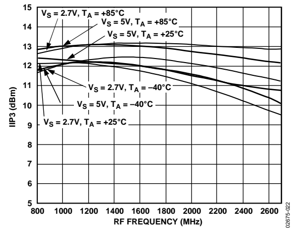
Figure 13. IIP3 vs. F_{LO} , V_{GIN} = 1.2\text{ V} , F_{BB} = 1\text{ MHz}
