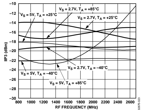
Figure 14. IIP3 vs. F_{LO} , V_{GIN} = 0.2\text{ V} , F_{BB} = 1\text{ MHz}
