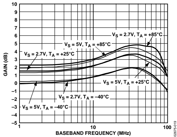
Figure 10. Gain vs. F_{BB} , V_{GIN} = 0.7\text{ V} , F_{LO} = 1900\text{ MHz}
