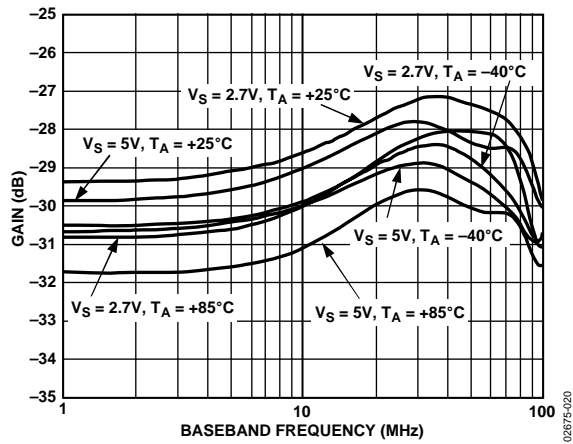
Figure 11. Gain vs. F_{BB} , V_{GIN} = 1.2\text{ V} , F_{LO} = 1900\text{ MHz}
