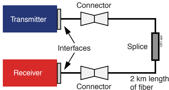
Figure 25. System design diagram.
