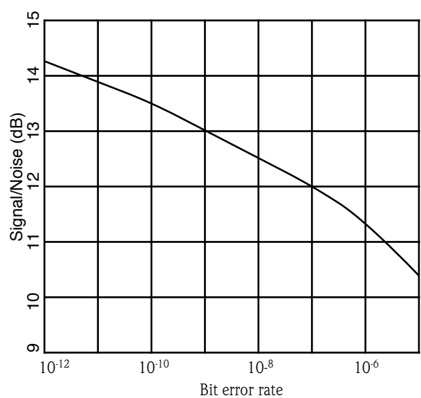
Figure 24. BER versus signal-to-noise ratio.
